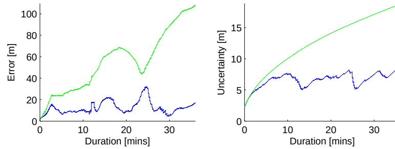
Fig. 3 Error (left) and 95% confidence (right) for the MLBL algorithm (blue) and the dead reckoning alone (green) for Experiment 1 where we have defined %90 confidence in terms of the largest eigenvalue of the covariance matrix.
