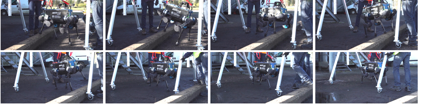
Fig. 6: Utopian trajectory executed on the real robot and oil rig scenario. Left to right and top to bottom: footsteps over slab, then fast trotting towards goal.
