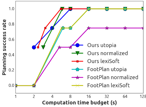
Fig. 2: Success rate of planning multi-controller (ours) and footstep-only (FootPlan) paths, for different computation time budgets and cost aggregation functions.
