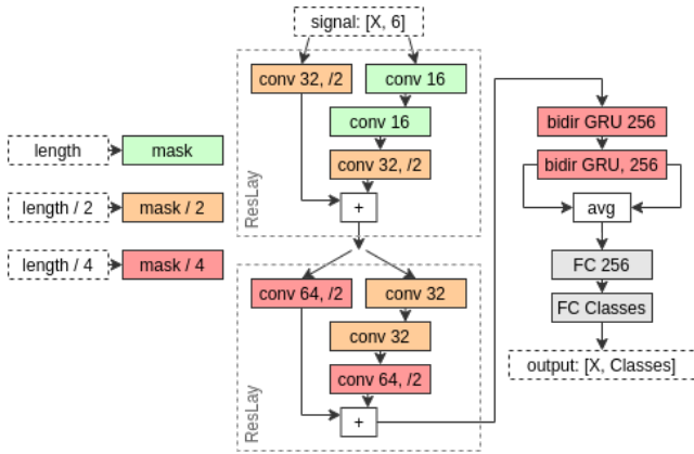
Fig. 5 Neural Network Structure used for Terrain Classification. The main blocks of neural architecture are convolutional (conv), recursive (GRU bidir), and fully connected (FC) blocks. The masking mechanism used in variable-length signal processing blocks takes appropriate masks, marked in green, orange, and red. These masks correspond to the individual signal lengths, taking into account the initial length and the reduction of size by convolution with stride equal to 2.
