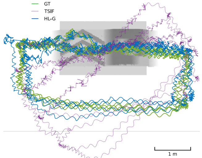
Fig. 7 Experiment 1, Trial 2: Top view of the estimated trajectories from TSIF (dashed purple), haptic localization (blue) and ground truth (green).
