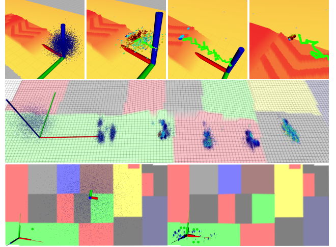
Fig. 14 Evolution of particle distributions during experiments. Particles are colorized by normalized weight according to the jet colormap (i.e., dark blue = lowest weight, dark red = highest weight). Top (Experiment 1): The green line indicates the ground truth trajectory. A) At start, all the particles have the same weight and are normally distributed at the starting position. B) After a few steps on the ramp, the robot pose is well estimated on x and z directions, but there is uncertainty on y . C) When the robot approaches the chevron the particle set divides into two clusters, indicating two strong hypotheses as to the robot pose. D) After a few more steps on the chevron, the robot is fully localized and the particles are tightly clustered. Middle (Experiment 3): As the robot walks from left to right, the particle cloud makes two terrain class transitions. As the robot crosses the first transition, the cloud becomes more narrow in the x direction as error along this axis is corrected. Bottom (Experiment 3): Top-down perspective with the robot estimate initialized in the middle of the map and the initial particle distribution spread out over the whole map. Within 5 steps the particle distribution has re-sampled over the correct green terrain patch. The green circles are the classified footsteps.
