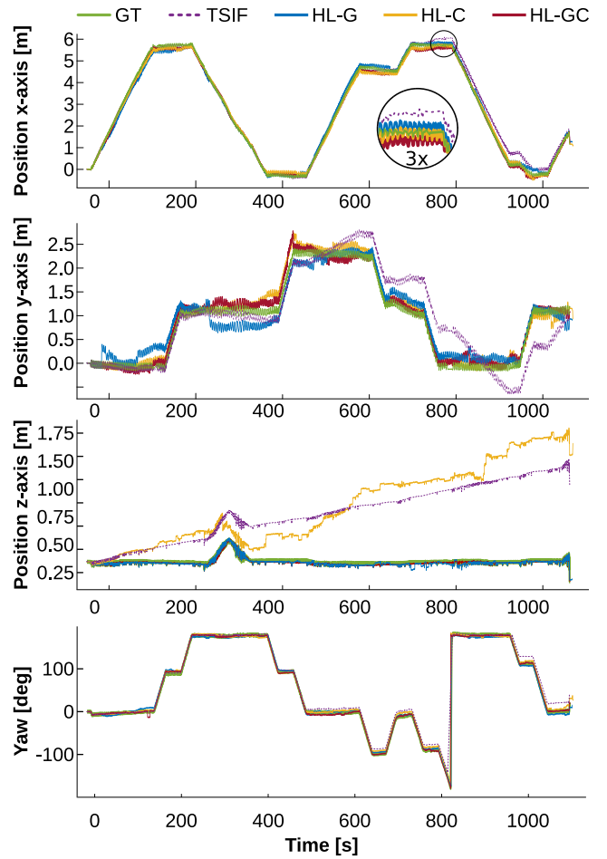
Fig. 12 Experiment 3, Trial 2: Here we show the difference in results when using only geometric information HL-G (blue), only terrain class information HL-C (yellow) and both HL-GC (red). We compare these to the state estimator (dashed purple) and ground truth (green).
