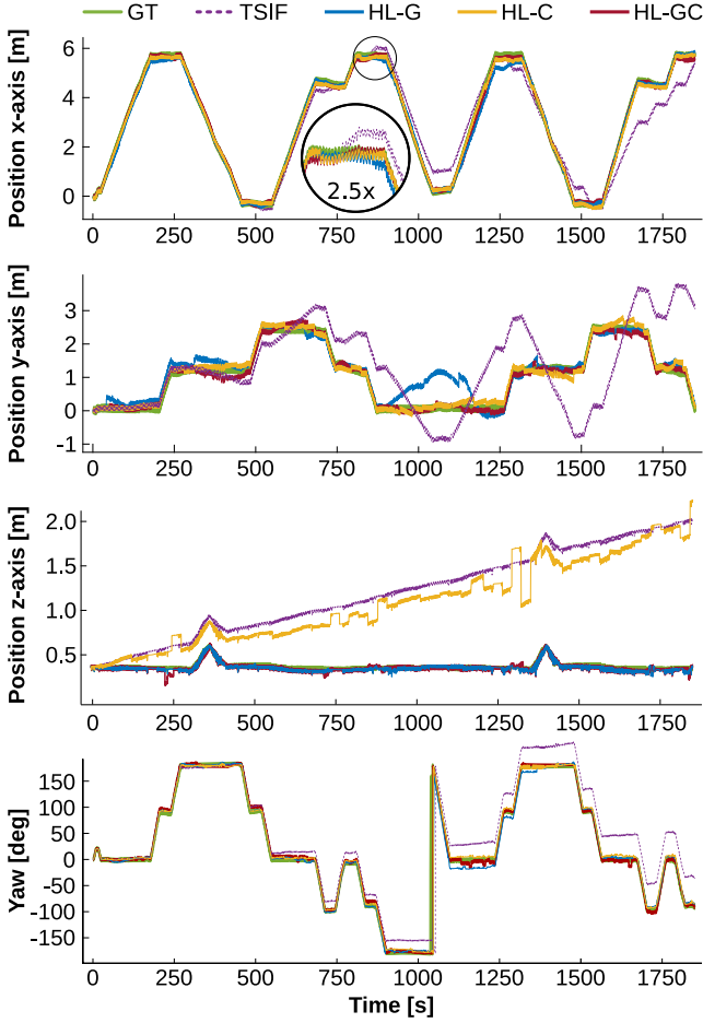
Fig. 13 Experiment 3, Trial 2: Here we show the difference in results when using only geometric information HL-G (blue), only terrain class information HL-C (yellow) and both HL-GC (red). We compare these to the state estimator (dashed purple) and ground truth (green).
