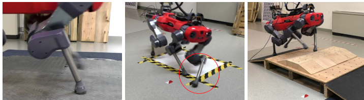
Figure 4: Lab experiments. Left: Robot foot compressing into soft terrain. Middle: Slip event while walking on slippery terrain. Right: Robot climbing over an obstacle.
