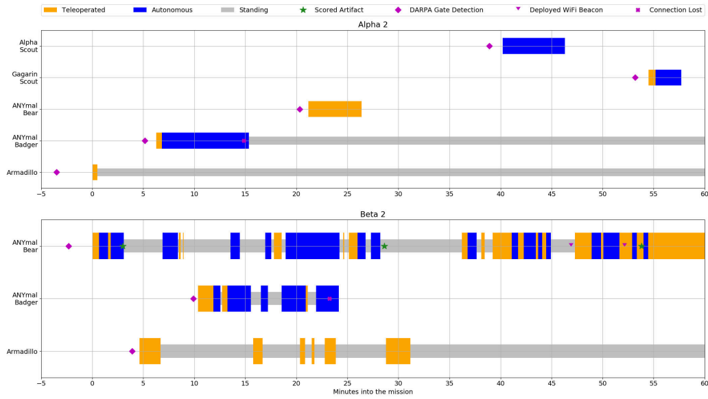
Figure 25: Mission analysis of Alpha 2 and Beta 2 runs. The plots show in which mode the robots were operating and when major mission events occurred. During the Alpha 2 run three robots were deployed in autonomous mode: The ANYmal Badger and the Alpha Aerial Scout could explore a significant part of the upper floor of the competition area, whereas the Gagarin Scout could plan its path through a series of staircases. ANYmal Bear was teleoperated downstairs a first set of staircases but could not proceed afterwards. At the Beta 2 run Aerial Scouts were not deployed due to narrow openings at the beginning of the course. The Armadillo rover was used to support the autonomous exploration of ANYmal Bear, while ANYmal Badger was sent to explore another area but got stuck on an obstacle and could not recover anymore. The last part of ANYmal Bear’s mission was supervised by the Human Supervisor due to an issue in its onboard state machine. ANYmal Bear scored three points by detecting and reporting artifacts to the DARPA Command Post. A video of the Beta 2 mission can be found at https://youtu.be/0-GbFrrWcL4 .
