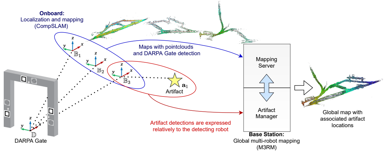
Figure 12: Illustration of the overall localization and mapping setup with coordinate frames for each robot \mathbb{B}_1 , \mathbb{B}_2 and \mathbb{B}_3 . All robots align themselves with respect to a common DARPA-defined coordinate frame \mathbb{D} using fiducial markers on the starting DARPA gate. The mapping server on the Base Station receives maps from the individual robots (blue) and combines them into a globally optimized map. Artifact detections, such as \mathbf{a}_1 , are recorded relative to the robot detecting them ( \mathbb{B}_3 ) and are sent to the artifact manager (red) for storing, additional inspection, and reporting them in coordinate frame \mathbb{D} using the globally optimized map to the DARPA Command Post for scoring.
