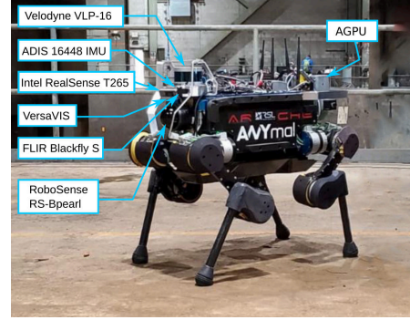
(b) Urban Circuit
