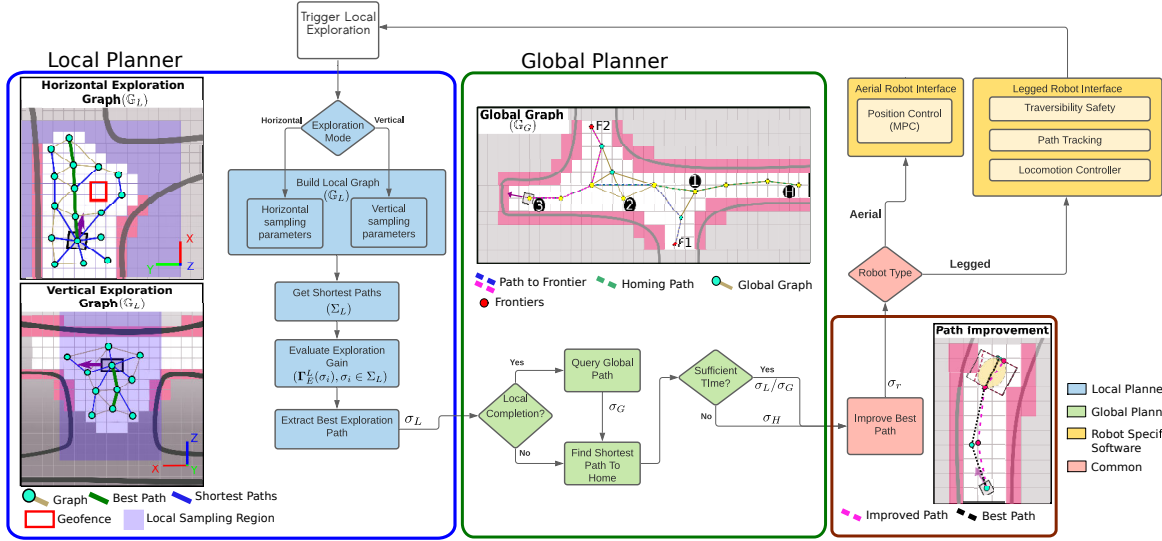
Figure 11: Functional diagram of the key functionalities of GBPlanner. This method bifurcates around a local and global planning mode with the first responsible for efficient exploration around the current robot location and the second responsible for re-positioning to frontiers of the explored volume in distant areas of the map, as well as auto-homing. Special functionality is provided for multi-level exploration, while the admissible paths account for collisions with 3D obstacles as well as “no-go” zones (geofences) that mark the non-traversable regions detected.
