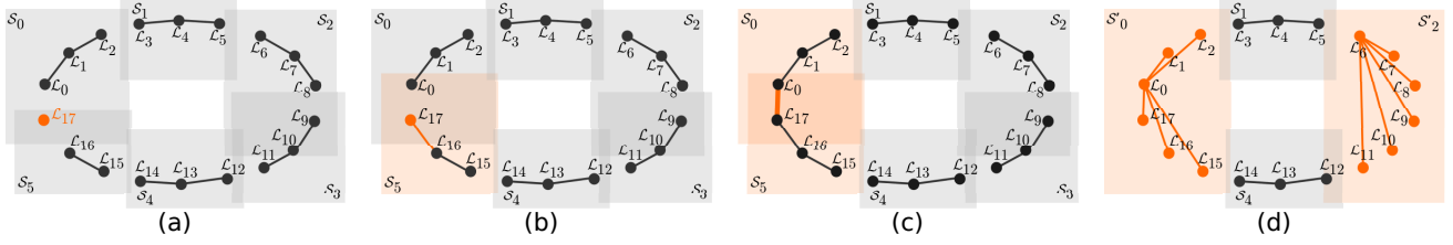
Figure 4: An example of scan integration and submap fusion. (a) There are 17 LiDAR scans \mathcal{L}_{0:16} (denoted by \bullet ) in the existing reconstruction. The scans are clustered into 6 submaps S_{0:5} , shown as rectangles ( \blacksquare ) which represent the AABB of each submap. \mathcal{L}_{17} ( \bullet ) is the latest new LiDAR scan, and there have been no loop closures. (b) Graph Clustering allocates \mathcal{L}_{17} to submap S_5 , and the new scan passes the Cloud Overlap Estimate (Sec. 3.1). Then \mathcal{L}_{17} is integrated into S_5 , expanding the AABB (as shown by \blacksquare ). (c) There is a new loop closure edge (orange line \text{---} ) given by the SLAM pose graph between \mathcal{L}_0 and \mathcal{L}_{17} . The head and tail of the loop closure connection define the submap overlap search range from S_0 to S_5 (shown in \blacksquare ). (d) Graph Clustering proposes the fusion of submaps S_5 and S_0 into S'_0 . Submap Overlap Estimate (Sec. 3.2) proposes the fusion between submaps S_3 and S_2 in S'_2 . If both proposals pass the Relative Uncertainty criterion (Sec. 3.3), fusion is executed and all submap indices are updated accordingly. The AABBs of S_0 and S_2 are therefore expanded (shown by \blacksquare ), but their accumulated submap clouds are not, as explained in Sec. 3.1.
