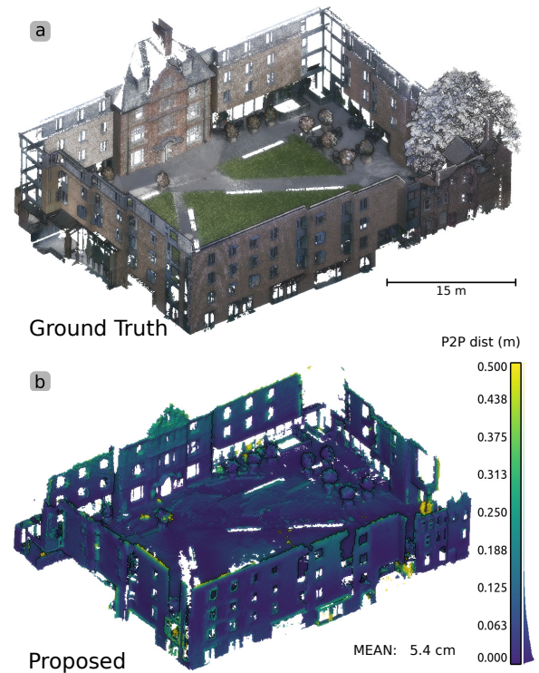
Figure 15: Exp 4.3 – Reconstruction of the proposed system (b) compared with the ground truth (a).
