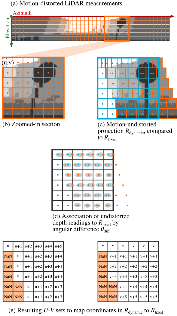
Figure 6: Motion aware LiDAR integration module to remap LiDAR points during dynamic motions. (a) – Motion-distorted LiDAR scan showing azimuth and elevation. (b) – Zoom in of a section. Each circle ● indicates a ray, with its corresponding cell in the grid. (c) – After motion undistortion, the undistorted projection R_{dynamic} (in orange ●) does not match the uniform grid (in light blue ●). (d) We iterate over the undistorted rays to find the closest ray assuming a uniform grid. (e) The output of the association are adjusted coordinates for azimuth ( U ) and elevation ( V ) angles of the undistorted projection.
