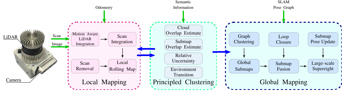
Figure 2: An overview of the proposed system that consists of a frontend ( Local Mapping ) and a backend ( Global Mapping ). Principled Clustering contains the proposed new strategies which estimate cloud and submap overlap, measure relative pose uncertainty in the SLAM graph, and leverage semantic information to detect transitions between indoor and outdoor environments. This module interacts with Local Mapping and Global Mapping to spawn new submaps (Sec. 3.1), propose or reject submap fusion (Sec. 3.2 and Sec. 3.3), and on-the-fly adjust reconstruction parameters based on semantic information (Sec. 3.4).
