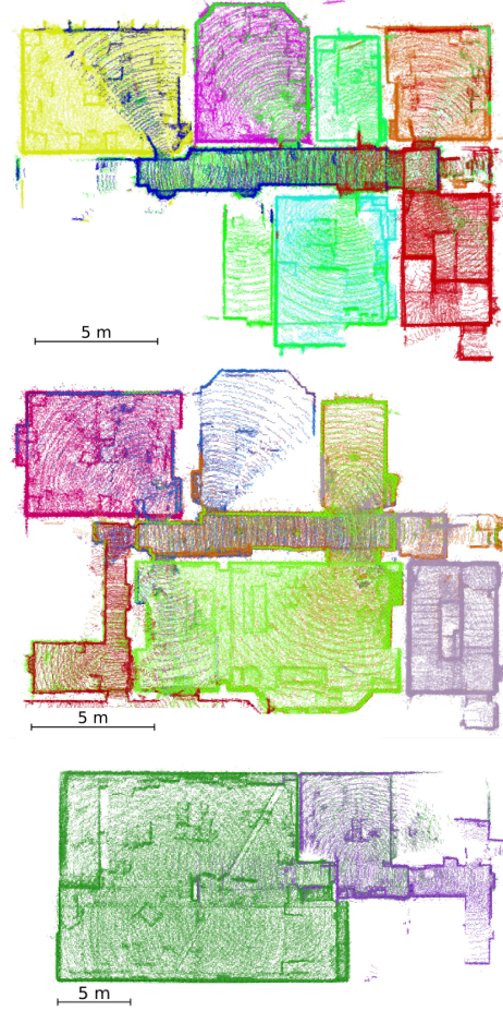
Figure 12: Exp 4.2 – The volumetric submap reconstructions of each floor ( Top: first; Middle: ground; Bottom: basement) in ORI, with each room segmented into unique submaps by the proposed system on the fly during exploration.
