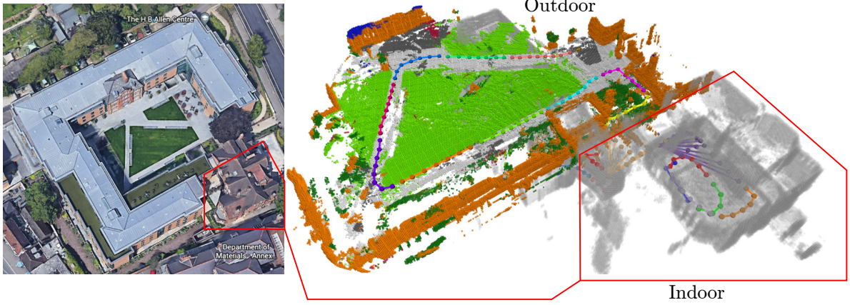
Figure 13: Exp 4.3 – Environment Classification: Parts of the constructed map that are classified as indoors (bottom right) are coloured in grey and parts of the map that are outdoors are coloured by their semantic labels. Lengths of the submaps (number of nodes) are also different between the two regions.
