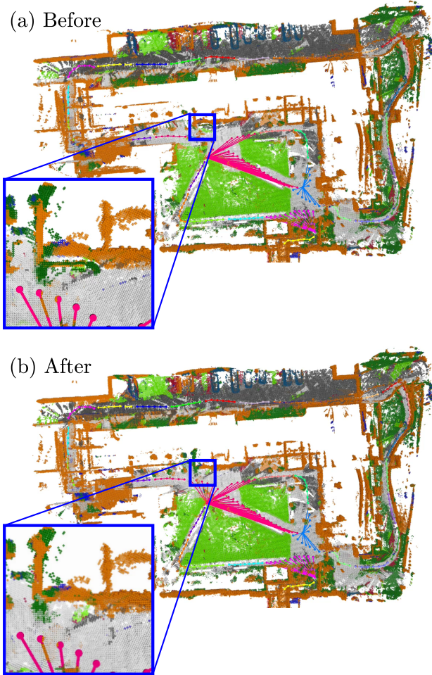
Figure 14: Exp 4.3 – Drift correction: (a) – the semantically annotated LiDAR reconstruction with building misalignment (orange) before loop closure; (b) – the elastic reconstruction after loop closure correcting the SLAM pose graph.
