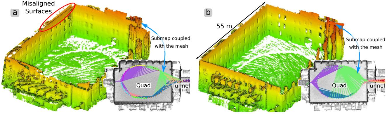
Figure 8: Exp 4.1 – The proposed spatial overlap analysis improves the global consistency in the reconstruction. Figure (a) and (b) present the mesh and volumetric representations of NCD Long experiment, created by the baseline and the proposed system, respectively. The volumetric representations are shown in grey overlaid with submap clusters. The mesh representations are created from the green submaps. Using spatial understanding of the environment leads to more reliable submap fusion and therefore better alignment. The mesh created by the previous pipeline has misaligned double surfaces while the proposed system improves the consistency in the mesh.
