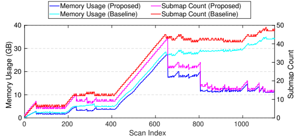
Figure 10: Exp 4.1 – The memory usage and submap counters of the proposed system and the baseline system in the NCD Long experiment.
