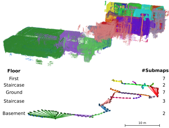
Figure 11: Exp 4.2 – The proposed system was tested in a multi-floor multi-room indoor environments. Top: The reconstruction result where each room is segmented by a submap indicated by a unique colour; Bottom: The clustered pose graph nodes using spatial overlap analysis on each floor.
