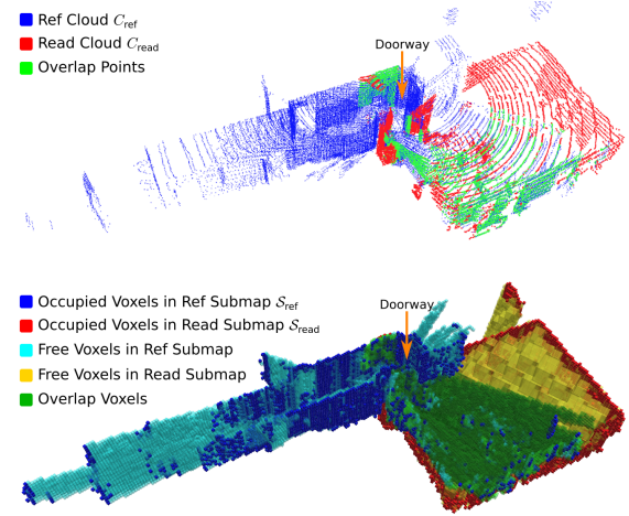
Figure 3: An example of Cloud Overlap Estimate and Submap Overlap Estimate. Top: Limited overlap between the reference cloud C_{ref} and the read cloud C_{read} when entering a room through a narrow doorway. Bottom: The voxel overlap between the volumetric occupancy reconstructions of the reference submap S_{ref} and the read submap S_{read} .
