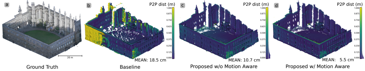
Figure 9: Exp 4.1 – The comparison between (a) the ground truth map of NCD Long experiment and each reconstruction created by (b) the baseline, (c) the proposed system without motion aware LiDAR integration and (d) the proposed system with motion aware LiDAR integration. Colours indicate point-to-point distances (P2P dist) between each reconstruction and the ground truth, and the distributions are also presented beside the colour bar.
