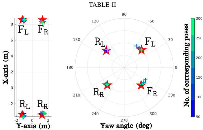
Fig. 4. Estimated t_x , t_y and \text{Yaw} for bus sequence-1 over different pose sizes. The GT calibration parameters are represented in red color.
