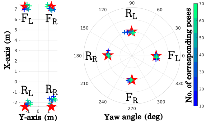
Fig. 5. Estimated t_x , t_y and \text{Yaw} for truck sequence-4 over different pose sizes. The GT calibration parameters are represented in red color.
