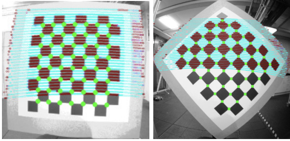
Fig. 17: Example calibration data samples used for the LiDAR to camera calibration. Hesai LiDAR points are overlayed on the image, and colored by each point’s intensity channel. The calibration target reflects the LiDAR beams with intensity contrast between the black and white squares seen in the camera image.
