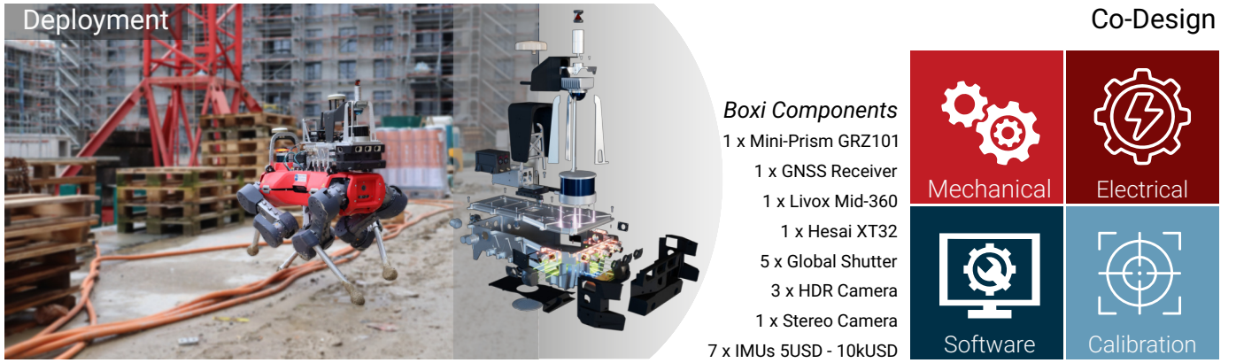
Fig. 2: Co-design of hardware, electrical systems, software, and calibration is essential for developing a robust sensor payload.
