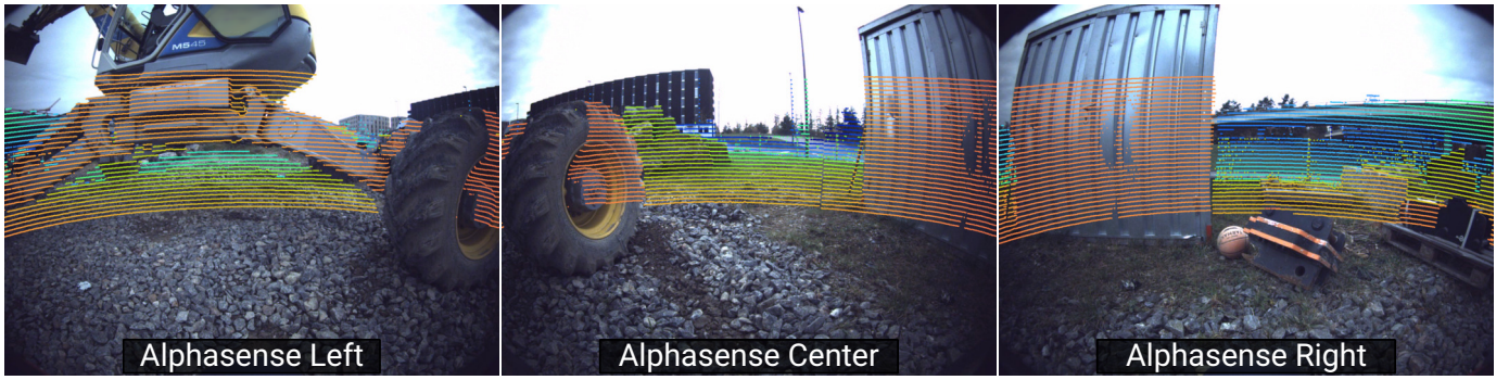
Fig. 21: Overlay of the LiDAR point cloud while moving forward at 1 \text{ m s}^{-1} , showcasing the consistency of the sensor calibration and the motion undistortion of the point cloud.
