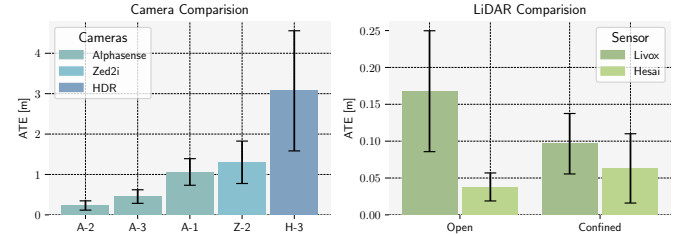
Fig. 4: Camera and LiDAR Comparison using OKVIS2 (HG4930) and DLIO (HG4930). (A-2, A-3, A-1, Z-2, H-3) indicates respective camera configuration (see Section IV-E). The Camera is evaluated on the Mountain Ascent dataset while the LiDAR comparison is provided on the Hike (Open) and Warehouse (Confined) datasets.
